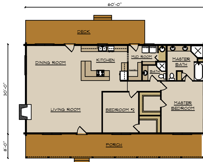
FLOOR PLAN
